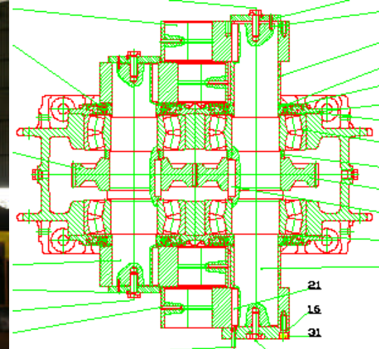
Cut-away of Vibrator
